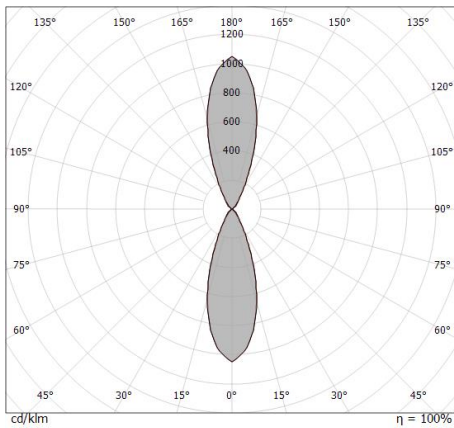
cd/klm — C0/C180 — C90/C270 η = 100%
